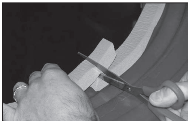
FIG.3 Trim Gasket
