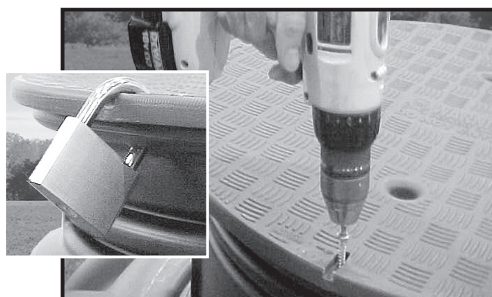
FIG.6 Secure Cover
